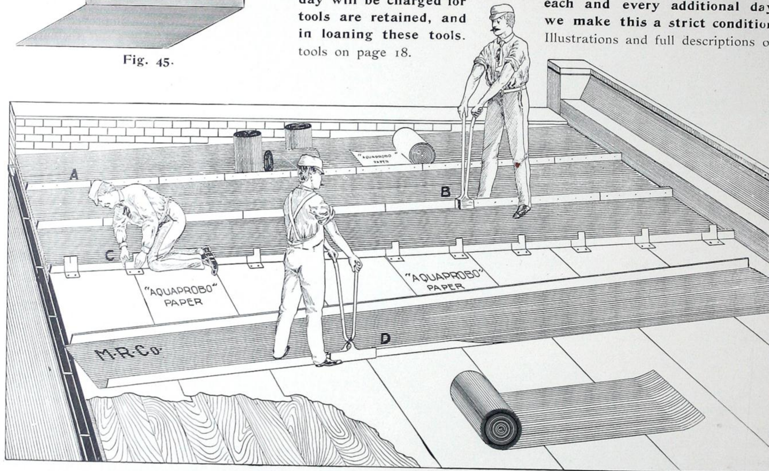
Fig. 46.—Ready Roll Cap Roofing in Process of Laying. A—Cap finished. B—Squeezing and Punching. C—Cleating. D—Turning up seam.
